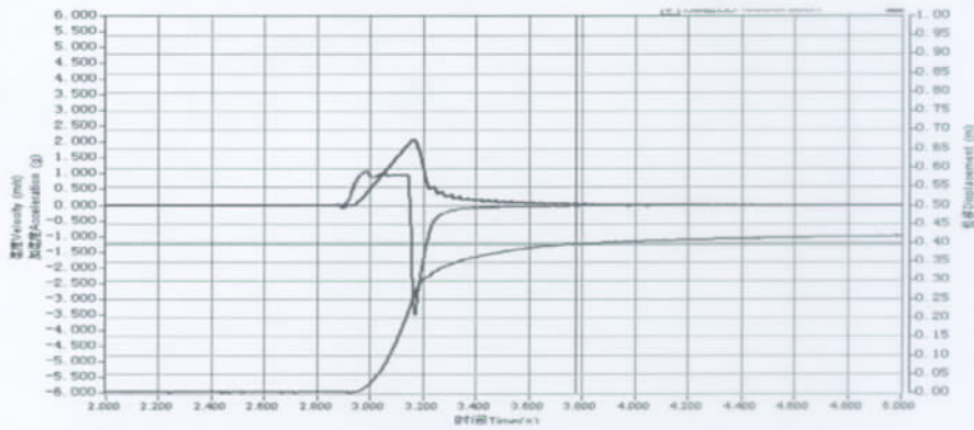
Test mass: 600kg, Rated speed: 1.75m/s
